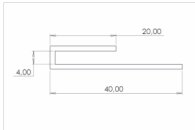
U-Display profile with tape for poster insertion
