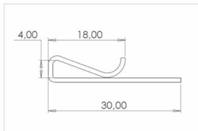
Poster holder with tape for poster insertion
